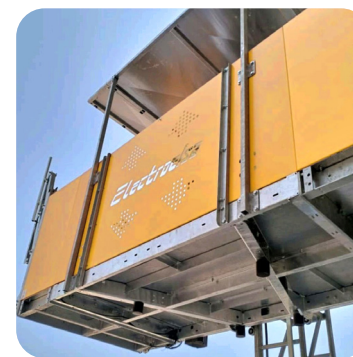
Material hoists
